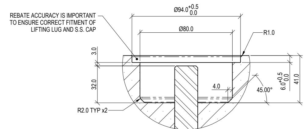
DETAIL C REBATE DETAIL SCALE 1:2
