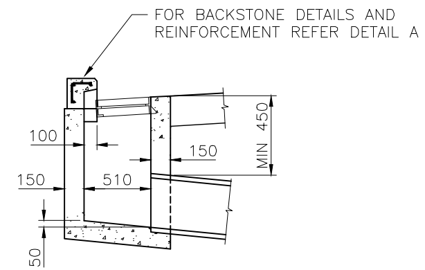
SECTION E-E
