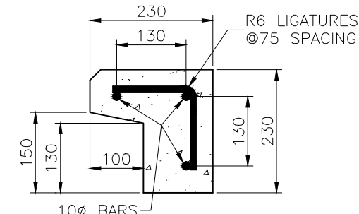
DETAIL A BACKSTONE TYPICAL SECTION
