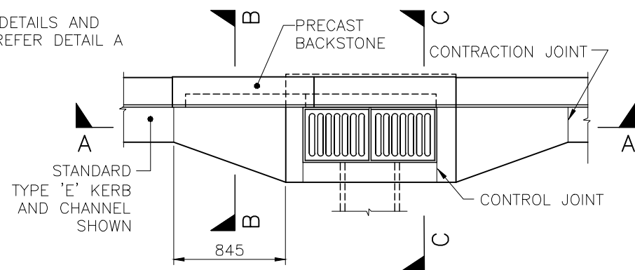
PLAN DOUBLE GULLY WITH EXTENDED KERB BACKSTONE
