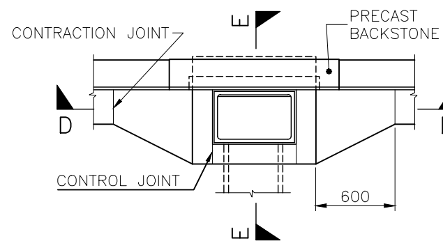
PLAN SINGLE GULLY
