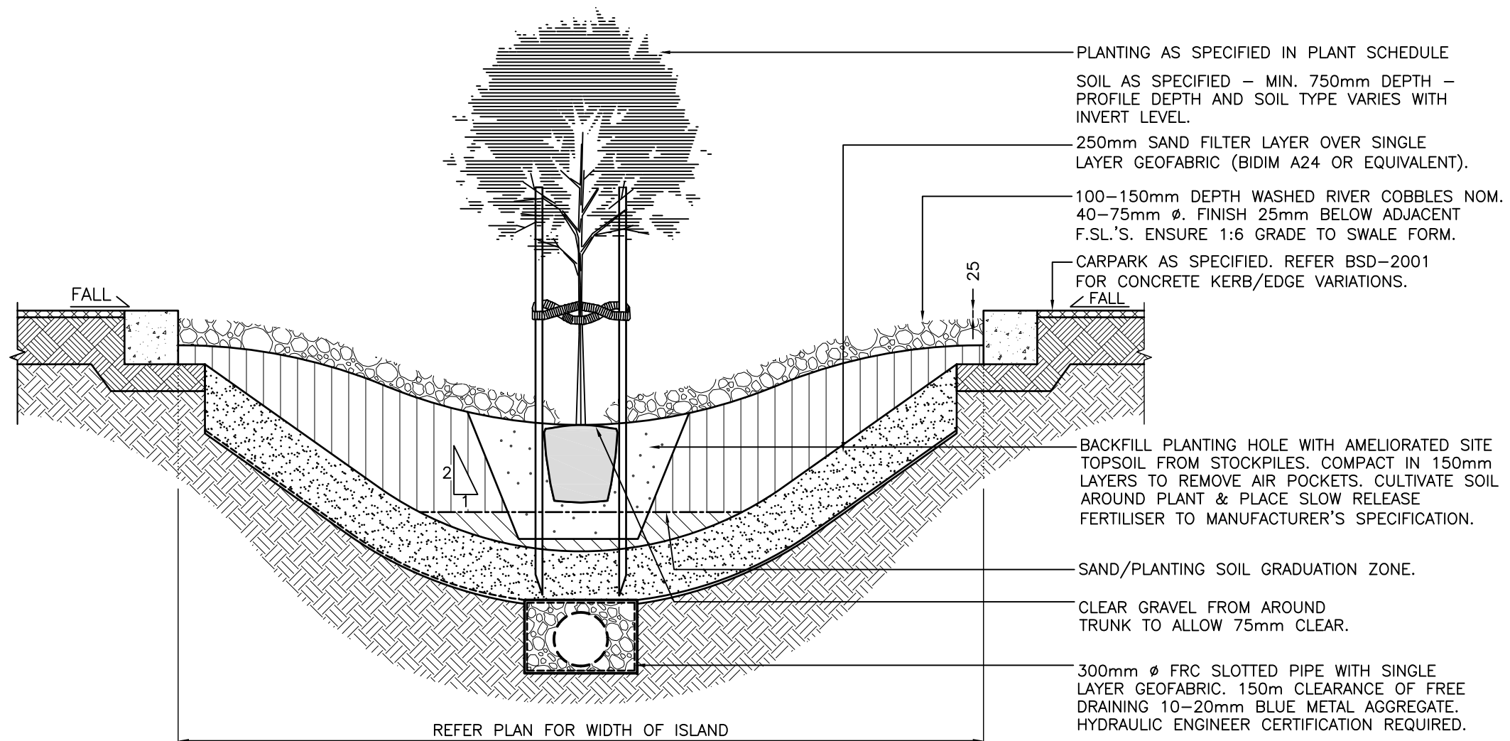
CARPARK BIO RETENTION SWALE WITH LANDSCAPING – SECTION
