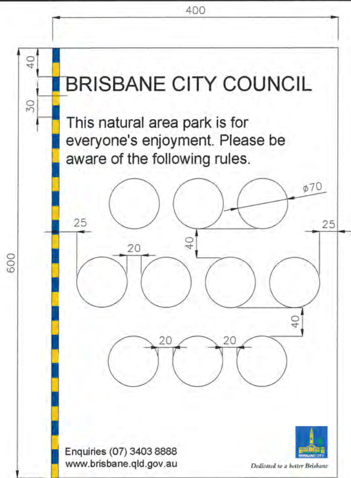
ORDINANCE SIGN PANEL SETOUT
