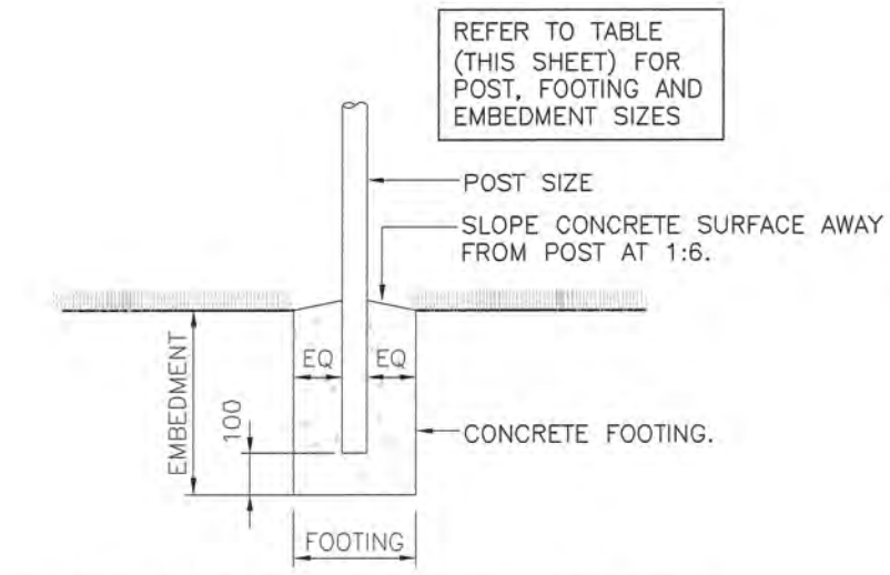
CONCRETE FOOTING DETAIL SCALE: 1:20
