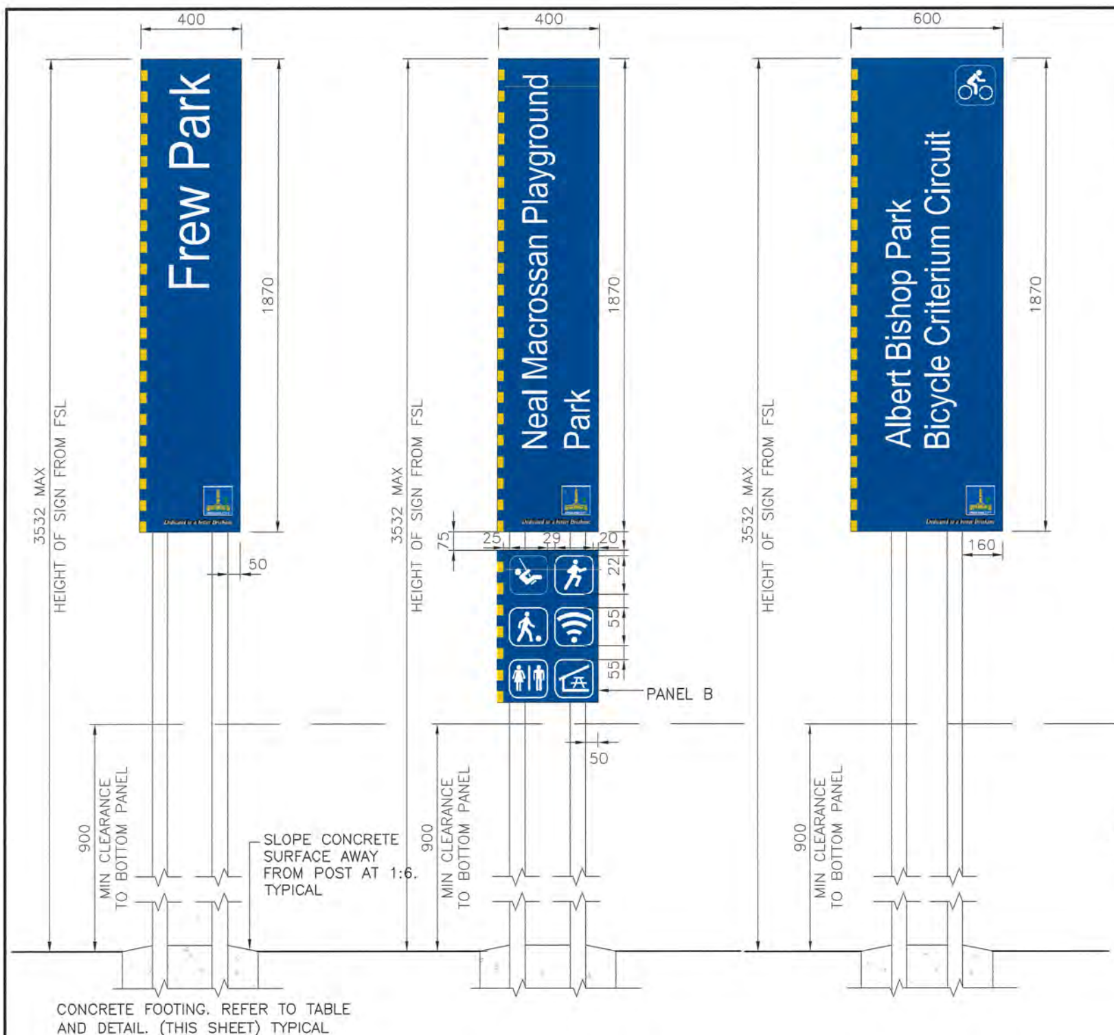
ALTERNATIVE 1 SCALE: 1:20 ALTERNATIVE 2 SCALE: 1:20 ALTERNATIVE 3 (SPECIFIC MAJOR PARK NODES ONLY) SCALE: 1:20
