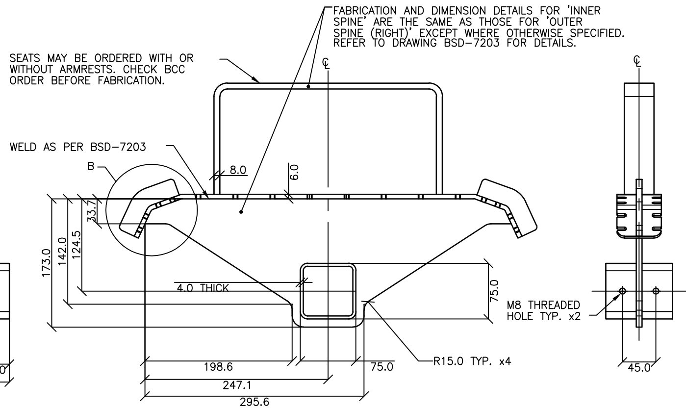
SIDE VIEW
