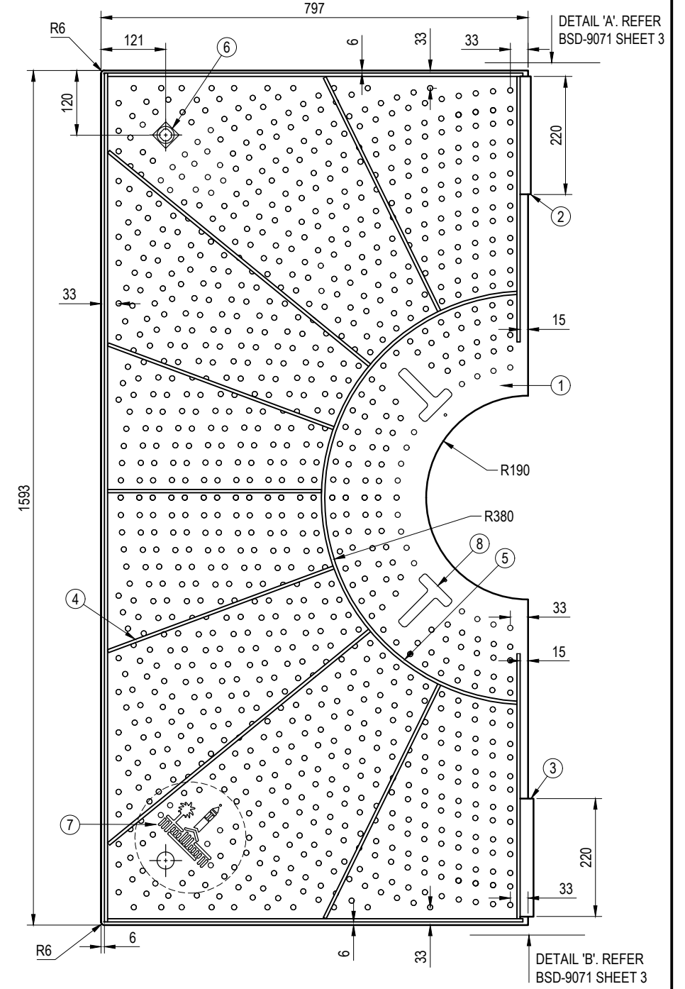
1600 x 1600 PLAN OF HALF GRATE - UNDERSIDE VIEW
