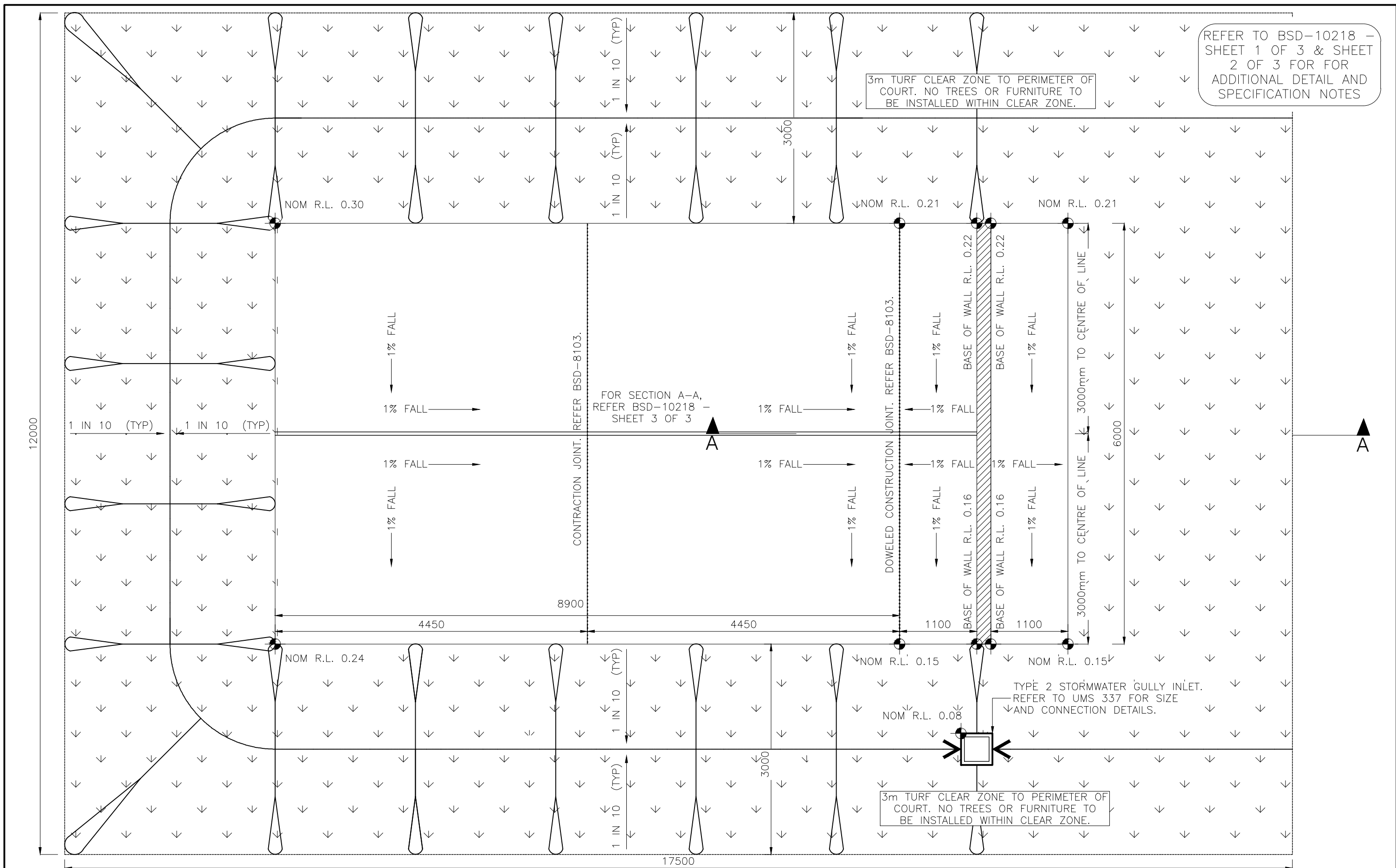
TENNIS REBOUND WALL – PLAN VIEW
