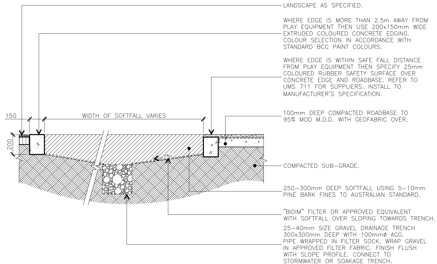
PLAYGROUND SOFTFALL – SECTION
