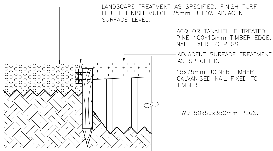
SECTION VIEW
