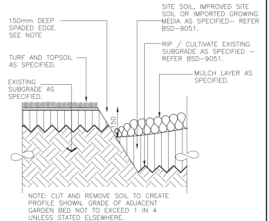
SPADE CUT GARDEN EDGE - SECTION
